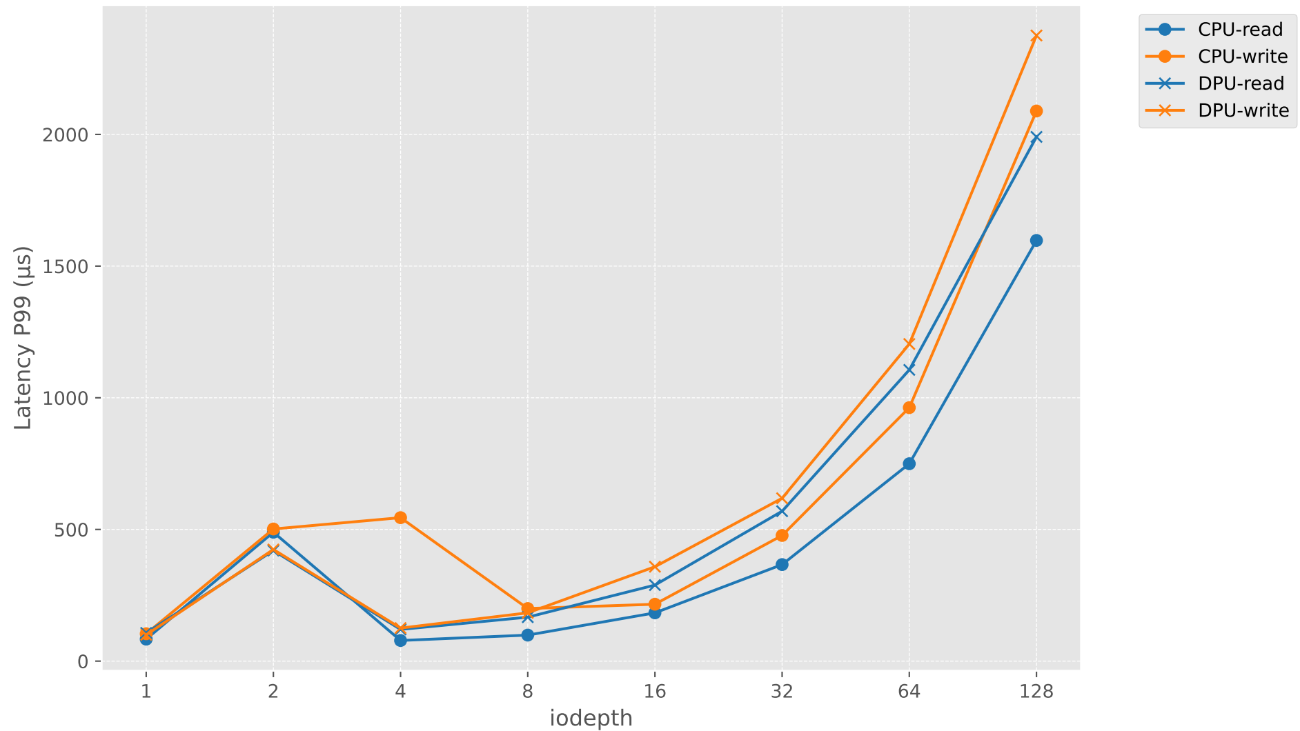
Latency P99 vs iodepth (Sequential)
